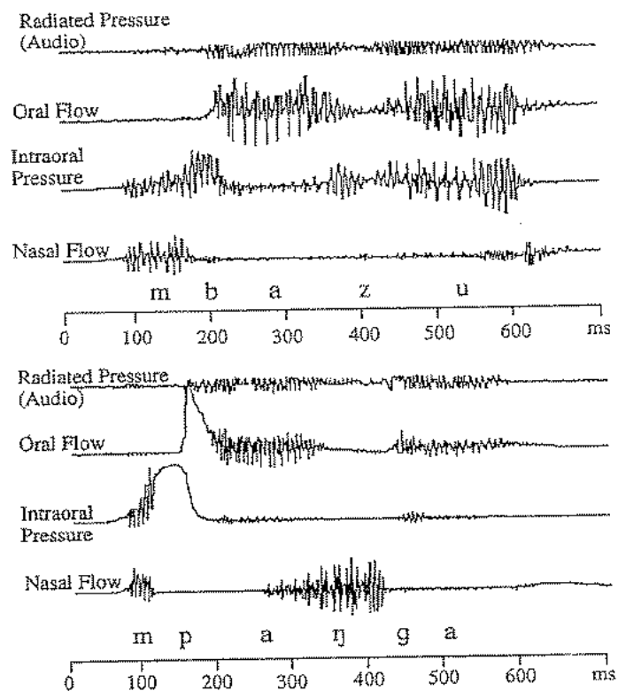
Figure 4.13 Aerodynamic records illustrating voiced and voiceless prenasalized stops in KeSukuma in the words mbazu 'goat' and mpagga 'alive (person)'. !
