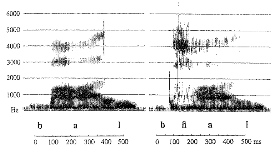
Figure 3.6 Spectrograms illustrating modal and breathily voiced stops in the Hindi words baɪ 'hair' and bʱaɪ 'forehead'.
