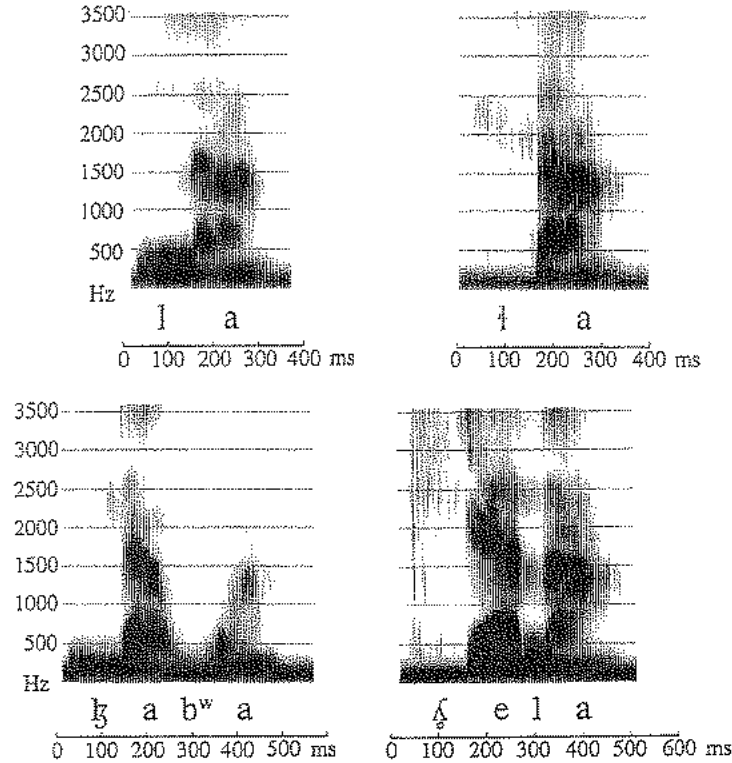
Figure 6.13 Spectrograms of four laterals in Bura. The words are la 'build', la 'cow', ɬab* a 'bear' and ɬela /ɬela/ 'cucumber'.
