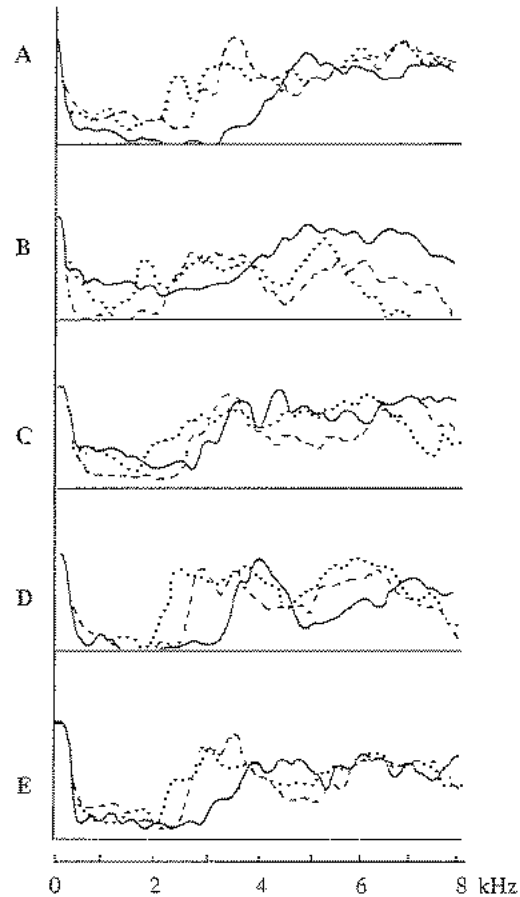
Figure 5.29 Spectra of Swedish s (solid line), ç (dashed line), and ş (dotted line) before a: as produced by five speakers designated A–E (after Lindblad 1980).
