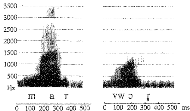
Figure 7.19 Spectrograms of the Ingush words mar 'husband' and vwɔɣ 'seven'
