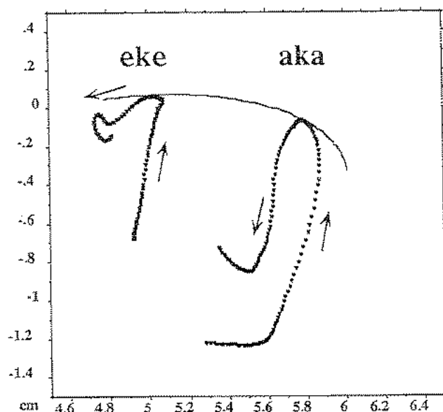
Figure 2.16 Movement trajectories for a point on the tongue rear (mean of 10 repetitions) during the Ewe words aká 'sarsil' and eké 'charcoal' (based on Maddieson 1993). Scales are in cm from arbitrary origins. Samples taken approximately 5 ms apart. A curve indicating the estimated location of part of the roof of the mouth has been drawn on the figure.
