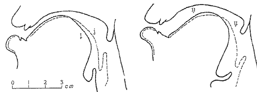
Figure 9.16 Tracings from x-ray cinematography films of Igbo vowels i as in òbí ( òbí in the standard Igbo orthography) 'heart'; i as in ùbí ( ùbí ) 'poverty of ability'; u as in ìbù ( ìbù ) 'weight'; and u as in òhù ( òhù ) 'it is'. In accordance with current IPA usage ̄ and ̃ are used to indicate Advanced and Retracted Tongue Root, respectively.
