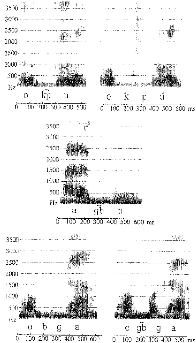
Figure 10.3 Spectrograms of words containing k̄p , ḡb , kp , bg and ḡbg in Eggon.
