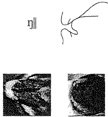
Figure 8.6 Palatogram and linguogram of a lateral click in the word ŋ||a?a 'scavenge' as spoken by a male Hadza speaker (speaker 2 in Figure 8.3 above).
