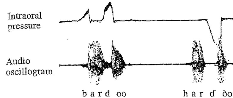
Figure 3.19 Intra-oral pressure records of the Hausa words bardoo 'longtailed dove' and hardoo 'Fulani man' (courtesy of R. Schuh).
