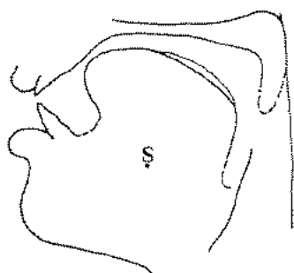
Figure 5.12 The articulatory gesture involved in Tamil \text{ɟ} in paɟa as indicated by x-ray data given in Svarný and Zvelebil (1955).
