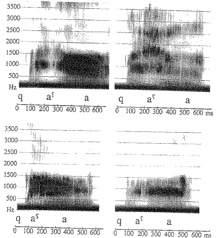
Figure 9.25 Spectrograms of the word qa'a as pronounced by four speakers of IX66, showing a pharyngealized vowel, followed by a non-pharyngealized vowel.
