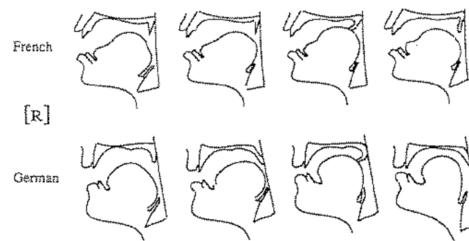
Figure 7.9 Frames traced from x-ray films of German and French intervocalic uvular trills (after Delattre 1971). The second frame in each row, shows retraction of the tongue, and the third frame in each row shows backward movement of the tongue root followed by tongue body raising and fronting of the uvula.
