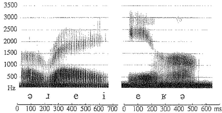
Figure 7.16 Spectrograms of rhotic approximants in a Southern British pronunciation of array , and a Standard German pronunciation of Ehre 'honour'.
