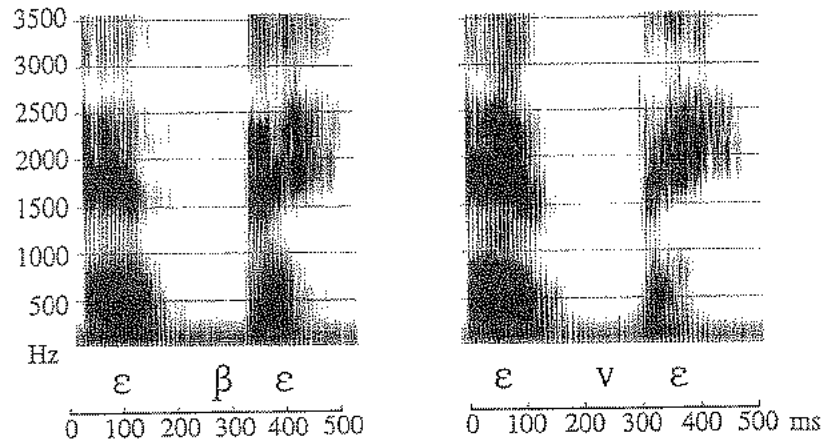
Figure 5.2 Spectrograms of Ewe bilabial and labiodental voiced fricatives in ɛβɛ 'people' and ɛvɛ 'two'.
