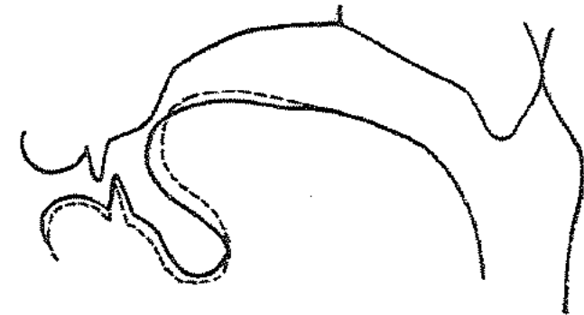
Figure 7.15 Mid-sagittal section of the Czech rhotics in the words para and maja based on palatographic and linguographic data (after Hála 1923). Solid line indicates r , dashed line ɹ .
