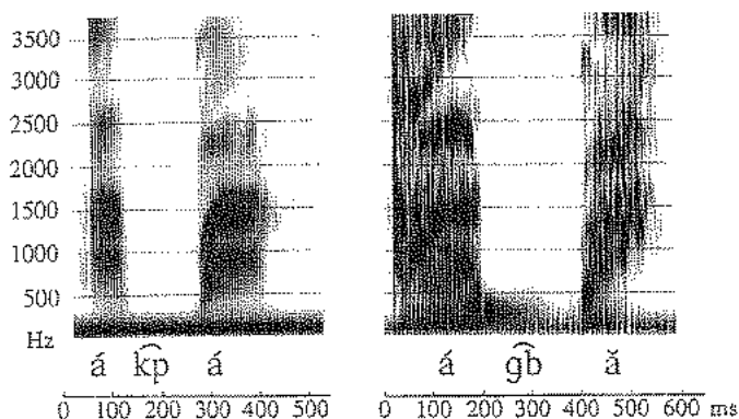
Figure 10.4 Spectrograms of \widehat{k}p in Efik \acute{a}\widehat{k}p\acute{a} 'river' and \widehat{g}b in Logbara \acute{a}\widehat{g}b\check{a} 'I hit'.
