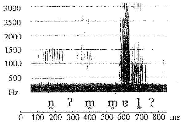
Figure 4.5 Spectrogram of the Columbian Salish word /n̥m̥aɪ/ 'lukewarm', containing two laryngealized nasals. The transcription below the spectrogram shows additional phonetic detail.
