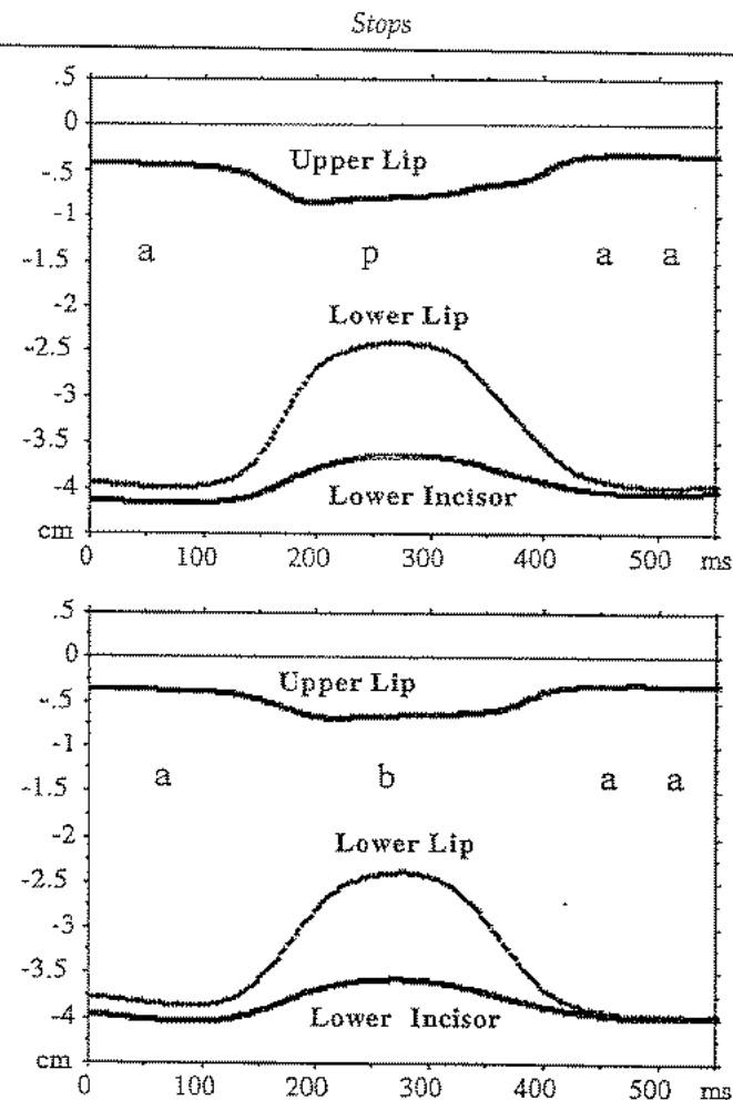
Figure 3.23 Vertical movement trajectories of the lips and jaw in production of apaa and abaa in Ewe. Mean of ten repetitions by one speaker (from Maddieson 1993).
