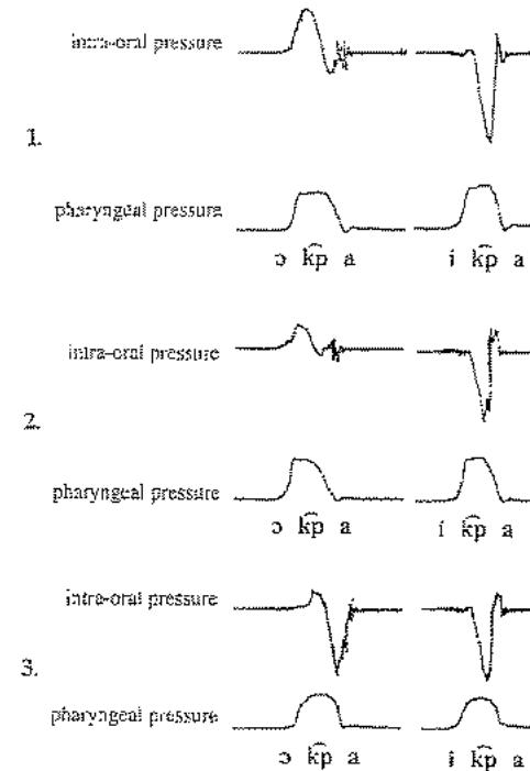
Figure 10.10 Aerodynamic records of the words \text{okpa} and \text{ikpa} extracted from three repetitions of an Edo sentence.
