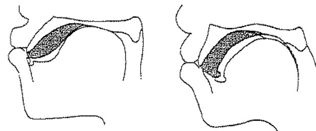
Figure 10.16 Tracings from x-ray films of [X66] bilabial clicks (based on Traill 1985). The shaded area shows the cavity between the two closures before the tongue is lowered. The position before release is shown by the lower tongue outline.
