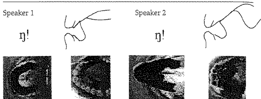
Figure 8.4 Palatograms, linguograms and inferred sagittal view of the alveolo-palatal click in the word 'cut' \eta!e?a 'cut' as spoken by two male Hadza speakers.
