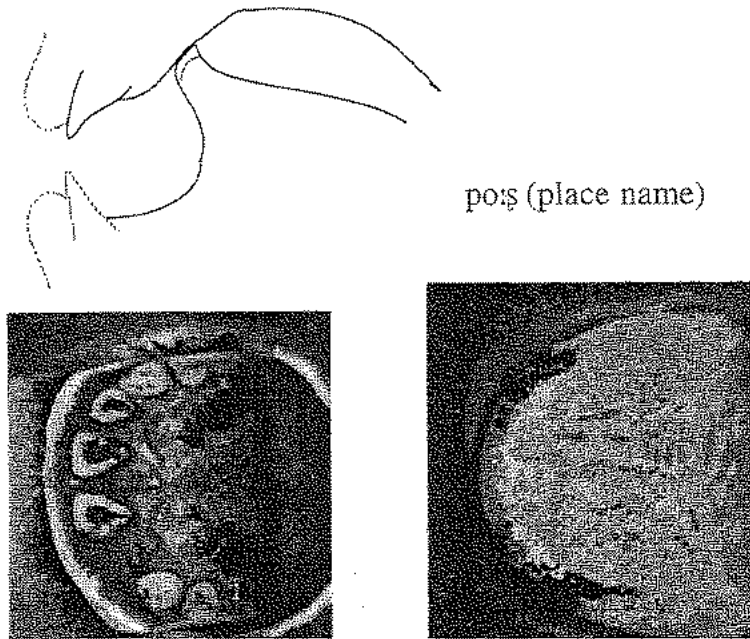
Figure 5.16 Palatographic and linguographic records of the Toda word po:ʃ (place name). The solid lines on the sagittal section show the known shape of the palate and the observed position of the sides of the tongue. Dotted lines indicate estimated positions of the lips and the center of the tongue.
