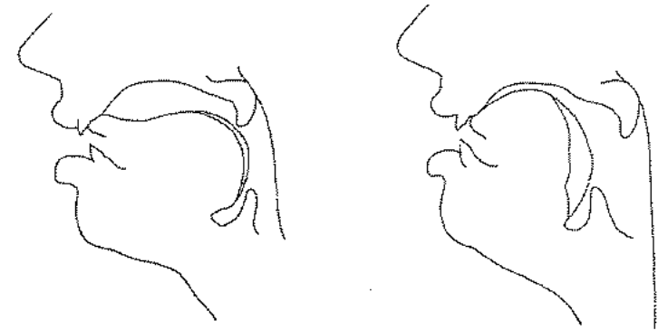
Figure 6.5 Cine x-rays of apical alveolar and laminal alveolar laterals in Russian: lak 'varnish', lina 'line' (based on data in Koneczna and Zawadowski 1956). The laminal articulation is the phonologically palatalized counterpart of the apical lateral.
