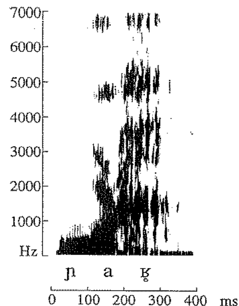
Figure 5.22 Voiceless uvular fricative trill \chi in Wolof (after Ladefoged 1968).
