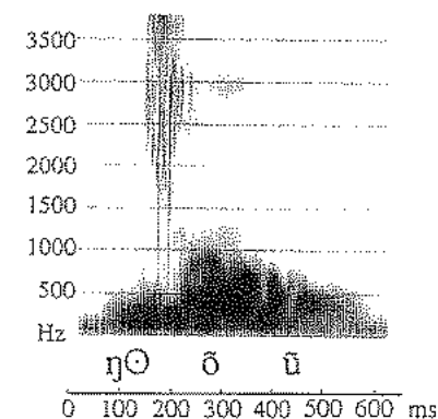
Figure 10.9 Spectrogram illustrating a nasalized bilabial click in #Hóá.
