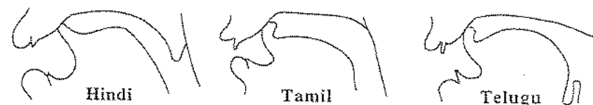
Figure 2.11 X-ray tracings of the apical retroflex \text{d̠} in Hindi and the sub-apical retroflex \text{ḍ} in Tamil and Telugu (after Ladefoged and Bhaskararao 1983.)
