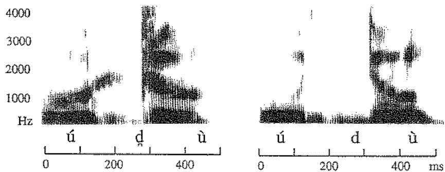
Figure 2.8 Spectrograms illustrating the difference between a laminal dental d and an apical alveolar d in Isoko in the words ú\grave{d}ù 'farm' and ú\grave{d}ù 'chest'.
