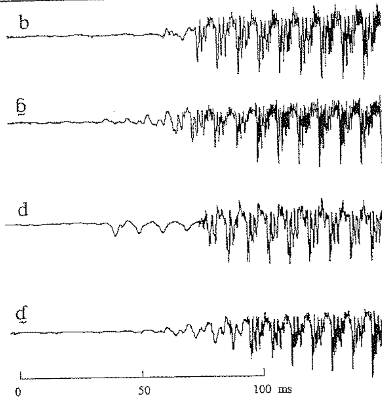
Figure 3.20 The difference between the releases of the modal voice and creaky voiced stops in Hausa.
