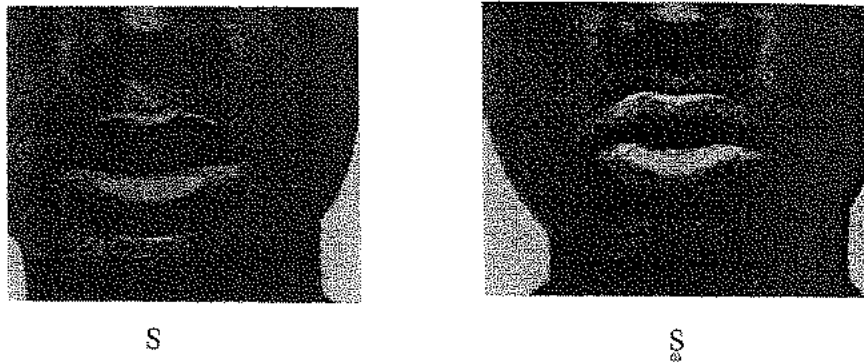
Figure 10.19 Lip photographs of Shona [s] and [ʂ] (after Doke 1931b).
