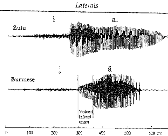
Figure 5.10 Waveforms illustrating differences between a voiceless lateral fricative in the Zulu syllable [a:] and a voiceless lateral approximant in the Burmese syllable [a:]. The lower amplitude and the anticipation of the voicing in the approximant are apparent.
