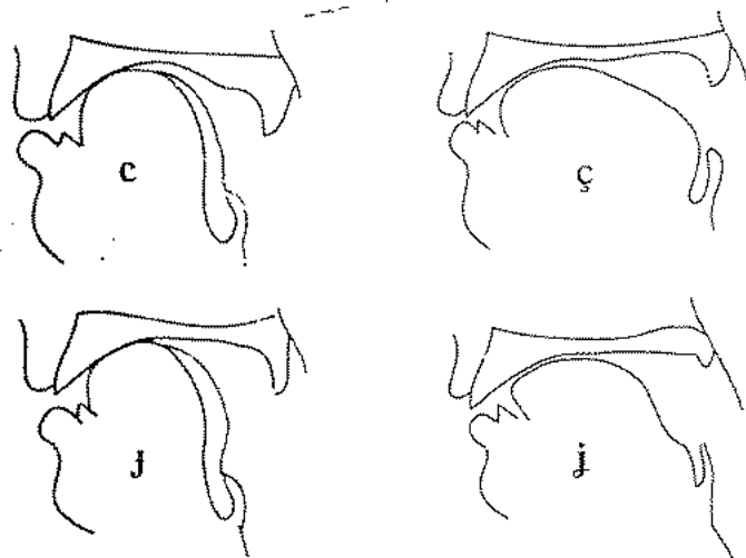
Figure 5.20 X-ray tracings of Hungarian palatals (after Bolta 1980). Note that the root of the tongue is more advanced for the stops on the left-hand side, than for the palatal fricatives ç and j on the right.
