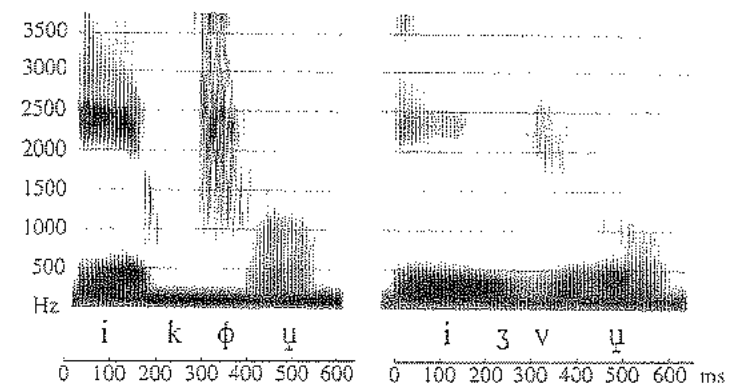
Figure 10.25 Spectrograms illustrating the effect of Kom fricative vowel y , inducing labiodental offglide of preceding consonants in the words iku 'death', and izu 'sky'.
