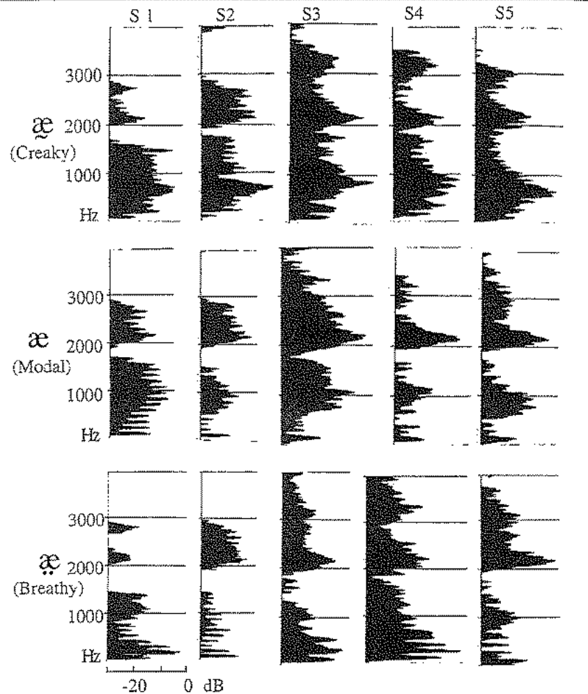
Figure 9.30 Narrow band power spectra of the creaky, modal and breathy vowels of five speakers of Jalapa Mazatec, taken during the middle of the vowels in the last row of table 9.15.
