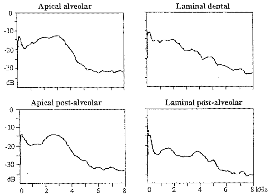
Figure 2.15 Mean spectra of the release bursts of the four Coronal stops of Eastern Arrernte. Each panel of the figure is calculated from ten tokens of words containing the stop in question in varied contexts.
