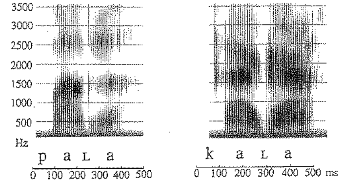
Figure 6.19 Velar lateral taps in the Melpa word pala 'fence' and the Kanite word kala 'dog'. Both speakers are male.
