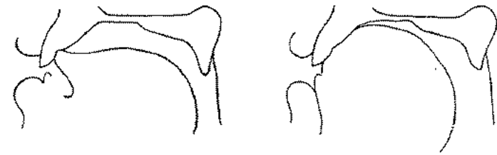
Figure 6.4 Cine x-rays of apical dental and laminal post-alveolar (palato-alveolar) laterals in Breton, Argol dialect: l in sa:la:n 'salads', l in butajadu 'bottles' (based on data in Bothorel 1982).
