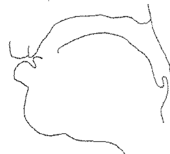
Figure 5.24 A voiceless epiglottal fricative ɸ (before ur ) in Arabic (from data in Bukshaisha 1985).
