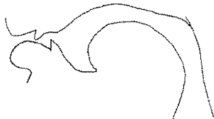
Figure 5.27 Swedish fj, a highly rounded, labiodental, velar or velarized fricative (based on data in Lindblad 1980).
