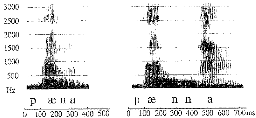
Figure 4.11 Spectrograms illustrating single and geminate nasals in Sinhala in the words pæna 'question' and pænnā 'jumped'.
