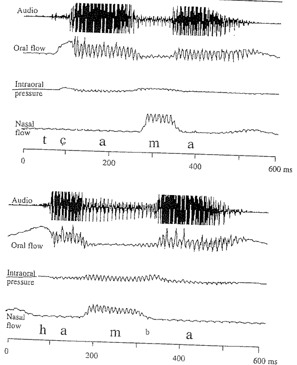
Figure 4.2 Aerodynamic records of Acehnese tcama 'sea-mew' and ham'ba 'servant'.
