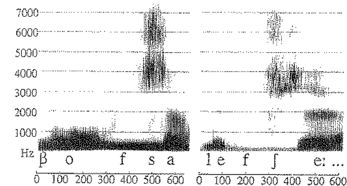
Figure 10.2 Spectrograms of the SePedi words \text{bofsa} 'youth' and \text{leffera} 'coward' spoken by a male speaker
