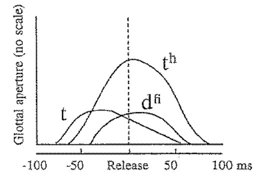
Figure 3.5 Glottal aperture in Hindi stops, based on fiberoptic data in Kagaya and Hirose (1975).
