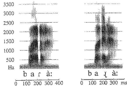
Figure 7.21 Spectrograms of the minimal pair bàrà: 'servant' and báɽà: 'begging' contrasting Hausa r and ɽ spoken by a male speaker from Kano.
