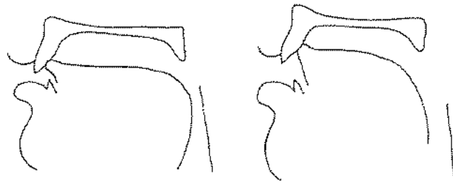
Figure 6.3 Cine x-rays of apical dental and apical alveolar laterals in Albanian: l in haja 'aunt', l in pala 'pair' (based on data in Bothorel 1969–70).
