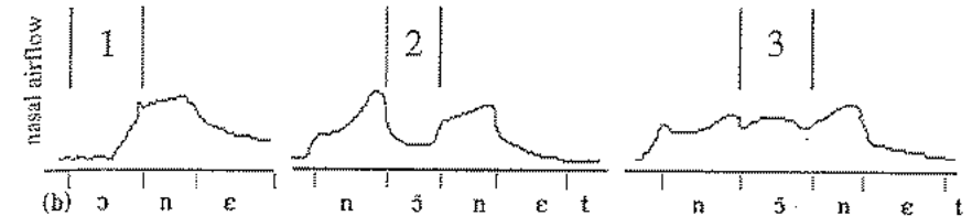
Figure 9.14 Records of nasal flow in three French words bonnet , nonnette , and non-être ('cap', 'young nun', 'non-entity'), showing the difference between oral, contextually nasalized and phonologically nasalized vowels (based on data in Cohn 1990).
