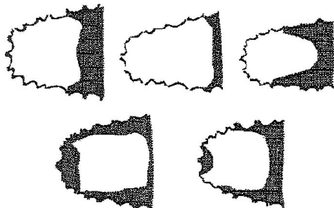
Figure 10.15 Palatograms of [X66] bilabial clicks from five speakers, based on data in Traill (1985). The three in the upper row show the only lingual contact to be in the velar region. The lower two have a tongue front contact as well as the labial and velar contacts and are those described as having "three points of articulation" by Traill.
