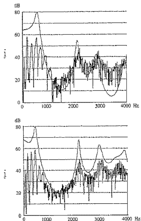
Figure 9.18 Spectra of the Degema vowels [ɨ] and [i].
