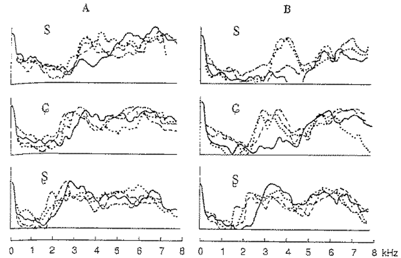
Figure 5.30 Spectra of Swedish s , ç , and ş before i (solid line), y (dashed line) and before u: (dashed and dotted line) as produced by two speakers A and B (after Lindblad 1980).
