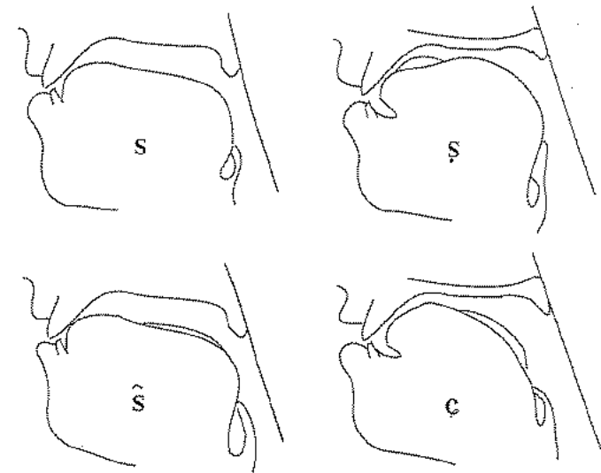
Figure 5.18 The four contrasting gestures for the sibilant fricatives in the Bzyb dialect of Abkhaz, based on x-ray tracings from Bgazhba (1964) and interpretive comments by Catford (ms in preparation).
