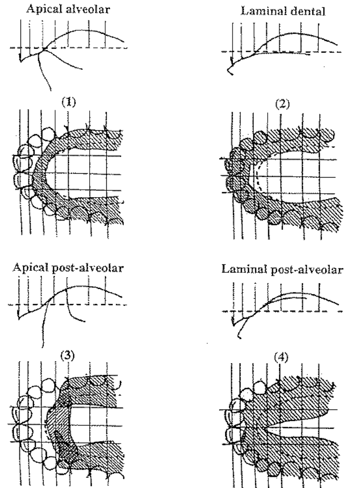
Figure 2.12 Palatograms and inferred articulatory positions for intervocalic coronal stops in Eastern Arrernte (courtesy of Andrew Butcher). The words illustrated are (1) atəmə 'burst', (2) atəmə 'grind', (3) kwəʃə 'smoke', (4) atəməʃə 'mother's father'.
