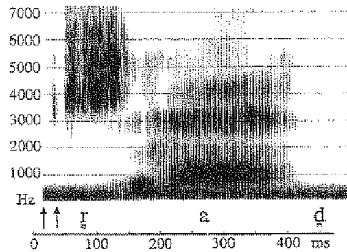
Figure 7.11 A spectrogram of the Czech word řad řad 'order'. The closure phases of each of the two vibrations of the blade of the tongue are indicated by arrows.
