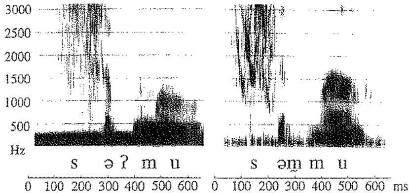
Figure 4.6 Spectrograms of s̥əʔm̥u 'mare' as pronounced by two speakers of Montana Salish. In both cases there is an epenthetic ə separating the first two consonants in the initial cluster.
