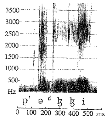
Figure 6.12 The sequence of lateral consonants in the first part of the Montana Salish word p'əllitʰtʰ 'turned over'. In the narrow transcription beneath the spectrogram the prepping is indicated by a raised 'd'.
