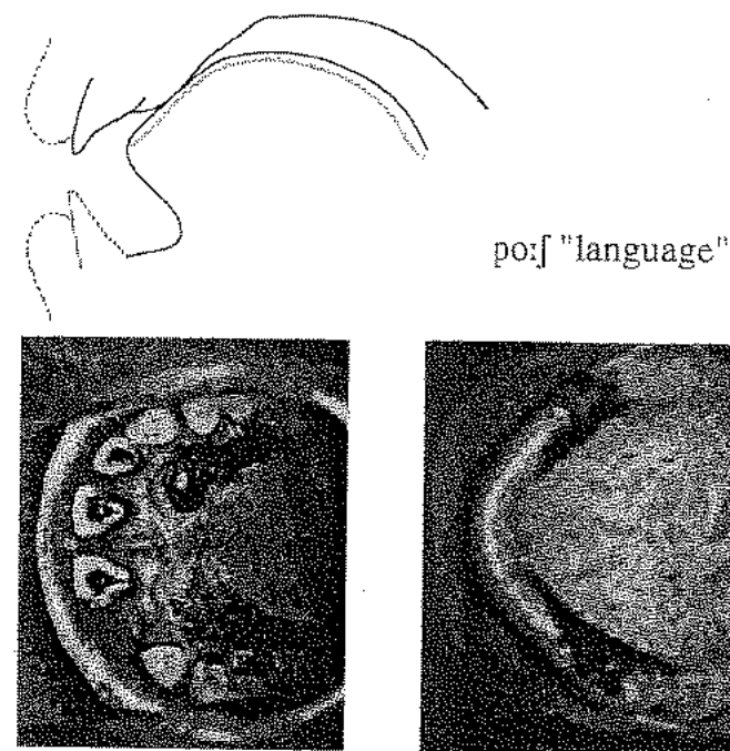
Figure 5.15 Palatographic and linguographic records of the Toda word po:ʃ 'language'. The solid lines on the sagittal section show the known shape of the palate and the observed position of the sides of the tongue. Dotted and grey lines indicate estimated positions of the lips and the center of the tongue.
