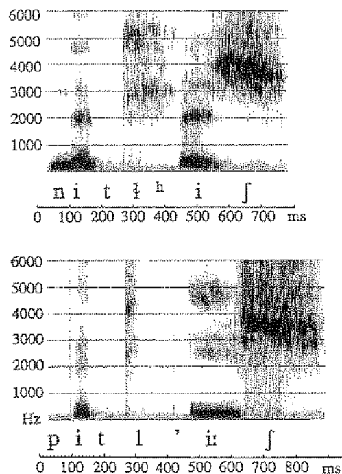
Figure 6.16 Navajo voiceless aspirated lateral affricate t^h in nitɬ 'it has arrived' and the ejective lateral affricate t^h in pitɬ 'his snake'.
