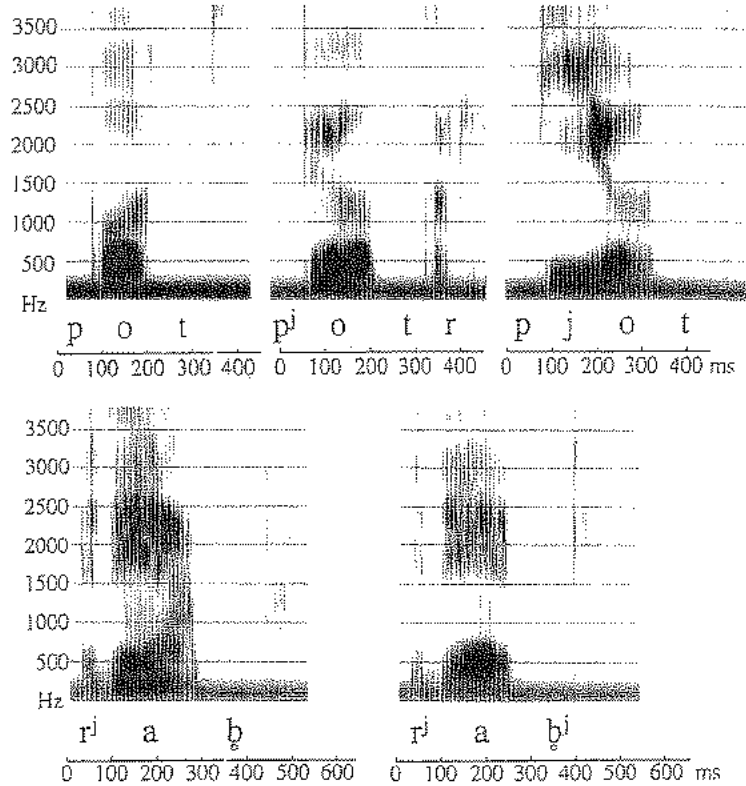
Figure 10.23 Spectrograms contrasting Russian plain and palatalized bilabial stops in the words pot 'sweat', pjotr 'Peter', riab 'pock-marked', and riab^j 'ripples' spoken by a male speaker from St Petersburg. The top line also shows the sequence pj in pjot 'drink' (3 sg.).
