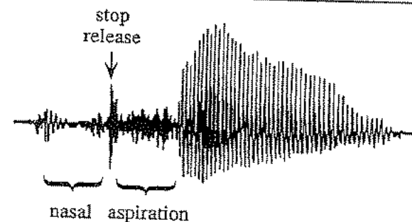
Figure 4.16 Waveform illustrating weak vocal cord vibration in devoiced nasal preceding aspirated stop in the Bondei word ntaa 'tilapia fish'.
