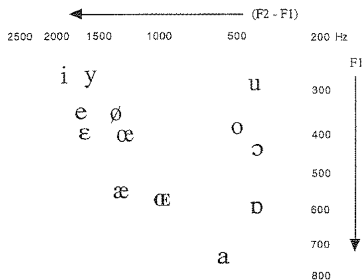
Figure 9.10 The mean formant frequencies of the long vowels of eight speakers of the Amstetten dialect of Bavarian (data from Trautmüller 1982).
