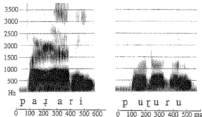
Figure 7.24 Spectrograms of rhotics in Warlpiri in the words pajari 'rainbow' and puṛuru 'hairstring'.
