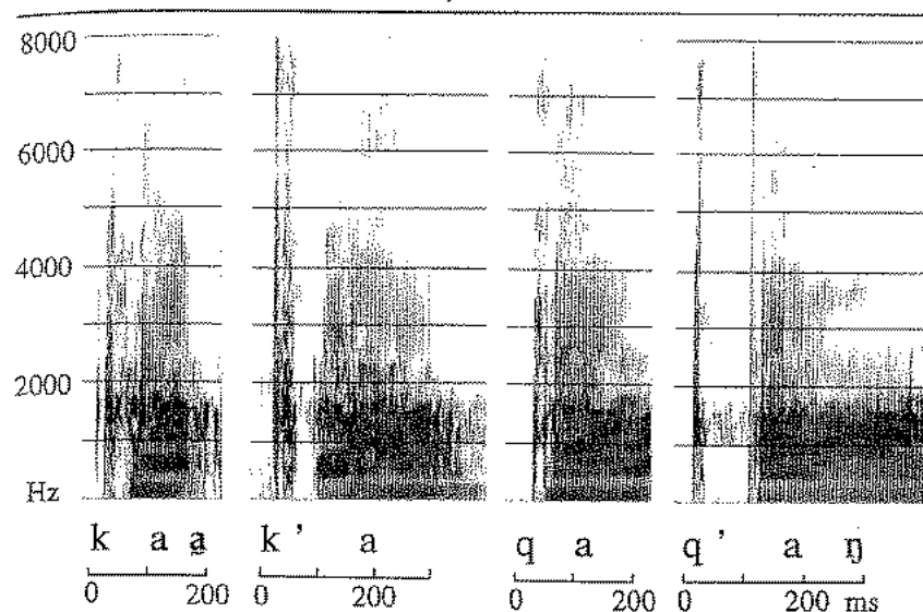
Figure 2.17. Spectrograms of contrasting velar and uvular plosives and ejectives in the K'ekchi words in Table 2.8.
