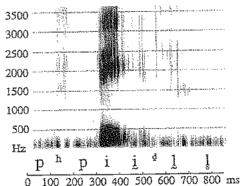
Figure 6.11 Spectrogram of the Montana Salish word ppi (in a narrow transcription [p h pij h l]) 'pint'.
