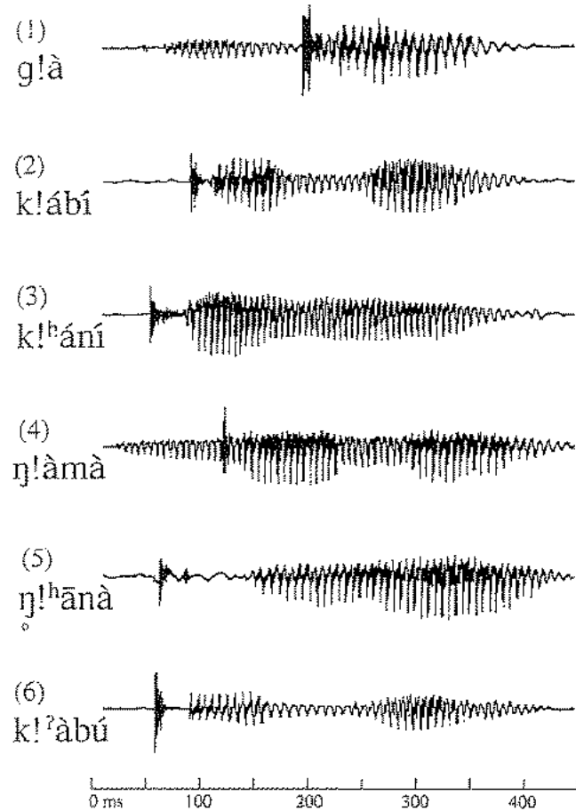
Figure 8.19 Waveforms of the first six Zhuǀ'hōasi alveolar clicks in table 8.5.
