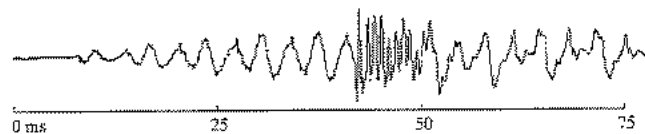
Figure 8.11 The waveform of a preglottalized nasaɪ click and the first few periods of the vowel in ɲ!àn. The time scale has been expanded so that the individual periods can be seen more easily.
