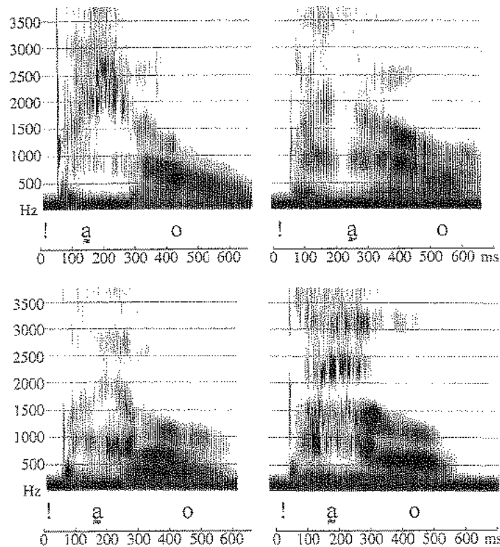
Figure 9.28 Spectrograms of the pronunciation of the word lao containing the low back strident vowel, spoken by four speakers of IXóó.
