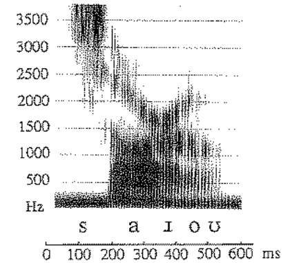
Figure 7.17 Spectrogram of American English sorrow saɹoʊ.
