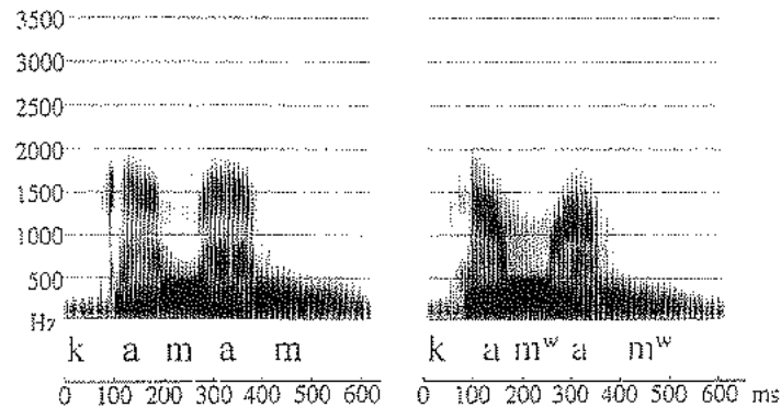
Figure 10.18 Spectrograms illustrating contrast of word-initial and final labialized bilabial plosives and nasals in Pohnpeian. The words are pal 'to hack', p w al 'to be silt', mars 'face', m w as 'worm', kap 'bundle', kap w 'new', kamam 'to enjoy kava', kam w am w 'to exhaust'.
