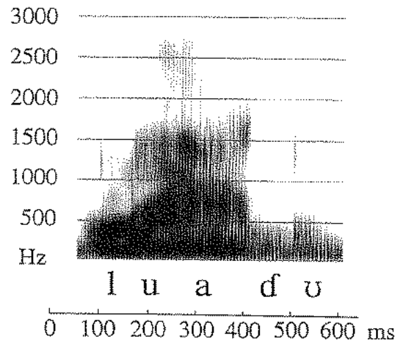
Figure 3.2 Spectrogram of the Ilwana word ladu 'speed'.
