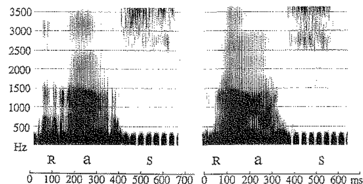
Figure 7.10 Spectrograms of uvular trills in two repetitions of raas 'breed' spoken by a male Southern Swedish speaker from Helsingborg.
