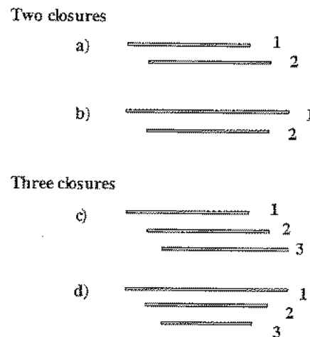
Figure 10.14 Some relative timing possibilities among multiple closures.
