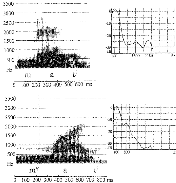
Figure 10.21 Spectrograms of the Marshallese words mat 'eye' vs m v at 'eel, worm', illustrating the contrast of plain and velarized nasals. Panels on the right show spectra of the nasal steady state. Frequencies of spectral peaks are indicated.
