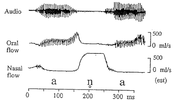
Figure 4.7 Aerodynamic records of the Burmese word (a) n̥a 'nose' that are typical of five of the six Burmese speakers.
