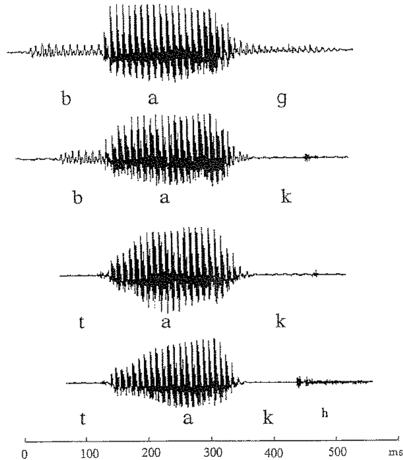
Figure 3.10 Waveforms illustrating contrasts among final velar stops in Eastern Armenian. The words are those in the final column of table 3.11.
