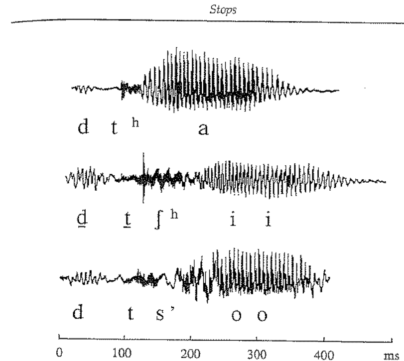
Figure 3.16 Waveforms of clusters with mixed voicing in Zhuǎhōasi.
