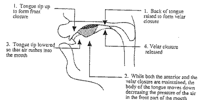
Figure 8.1 The articulatory sequence involved in production of an alveolar click in !Xóó. The dark shaded area shows the cavity enclosed when the closures are formed. The light shaded area shows the cavity just before the release of the anterior closure. The dashed lines show the lowered tongue positions corresponding to steps 3 and 4.
