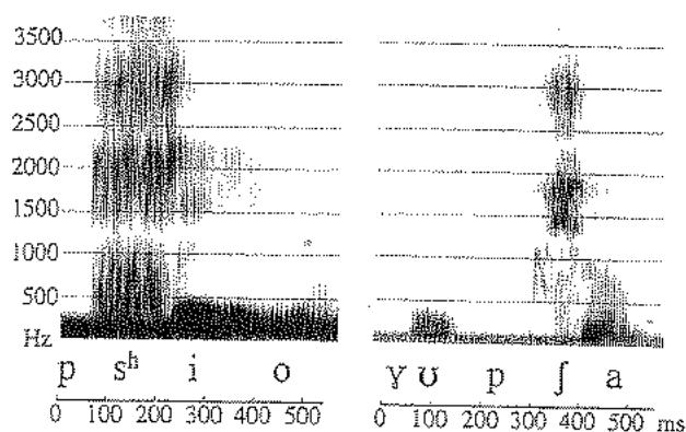
Figure 10.17 Spectrograms of the SePedi words ps^hio 'kidney' and yupfa 'to dry up'.
