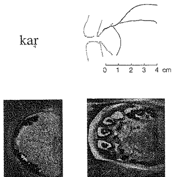
Figure 7.6 Palatogram, linguogram and reconstructed tongue position of the trill in the Toda word kar 'border of cloth'. The dark marks on the teeth in this and the following Toda palatograms are stains, and do not reflect tongue contact.
