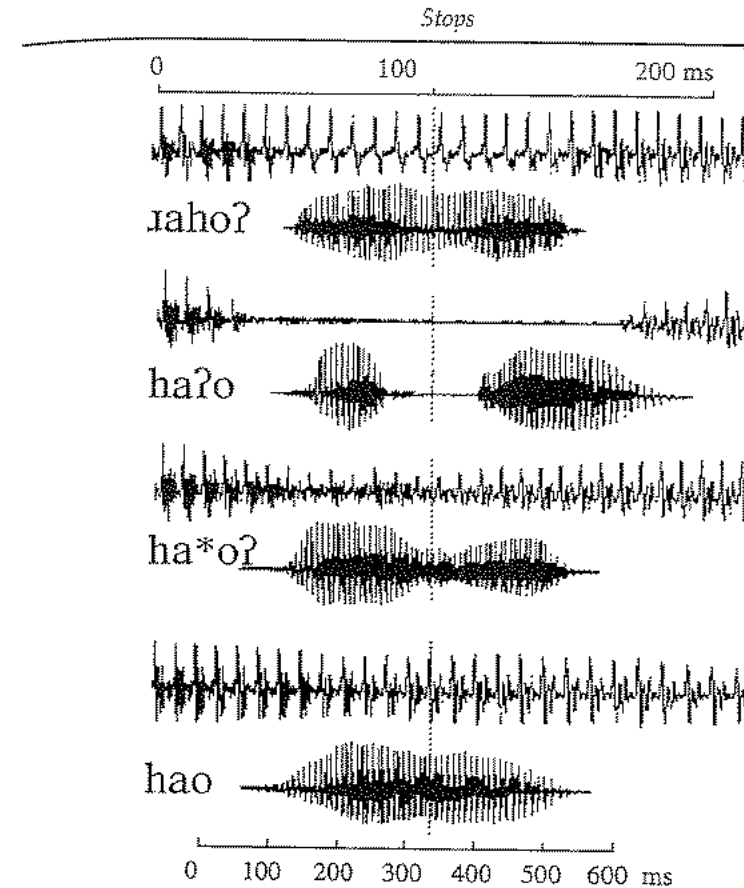
Figure 3.14 Waveforms of the Gimi words in Table 3.15. An expanded version of the intervocalic portion is shown above the waveform of the whole word, time-aligned as indicated by the dashed lines.
