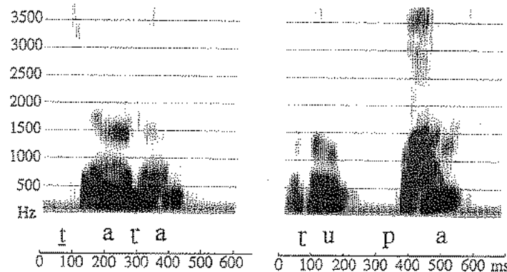
Figure 7.25 Spectrograms of flaps in initial and medial position in Warlpiri in the words tara 'sleep' and tupa 'windbreak'.
