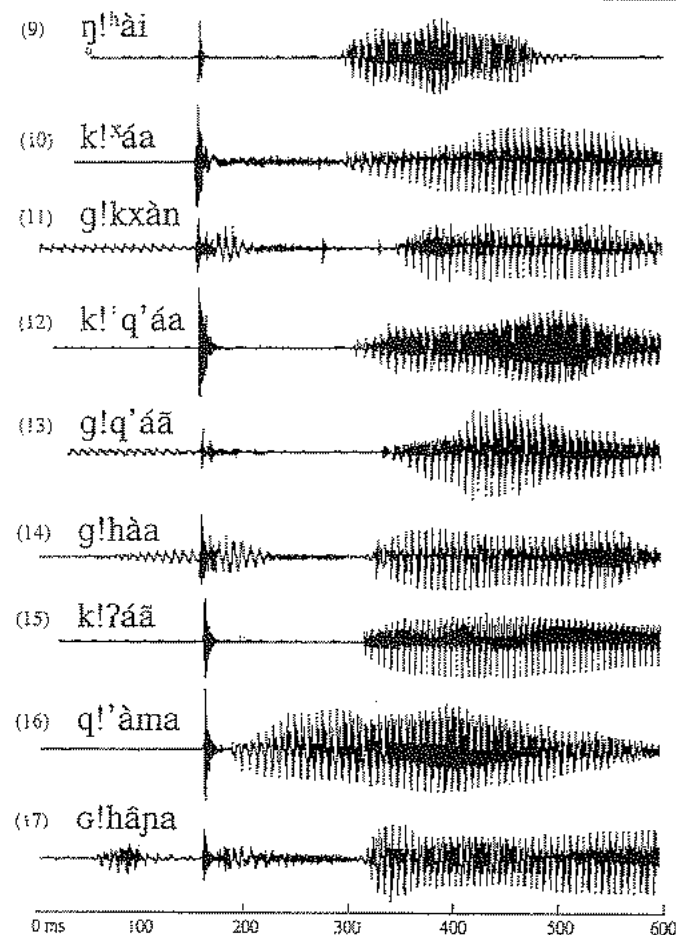
Figure 8.12 Waveforms showing the last nine alveolar clicks in !Xóó in table 8.4.
