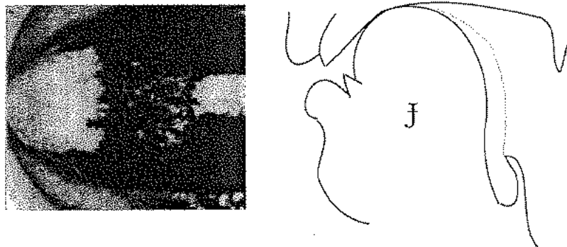
Figure 2.15 Linguogram and x-ray tracing of Hungarian voiced palatal stop (after Bolla 1980). The black tongue outline is the midline; the grey line shows the edge of the tongue.
