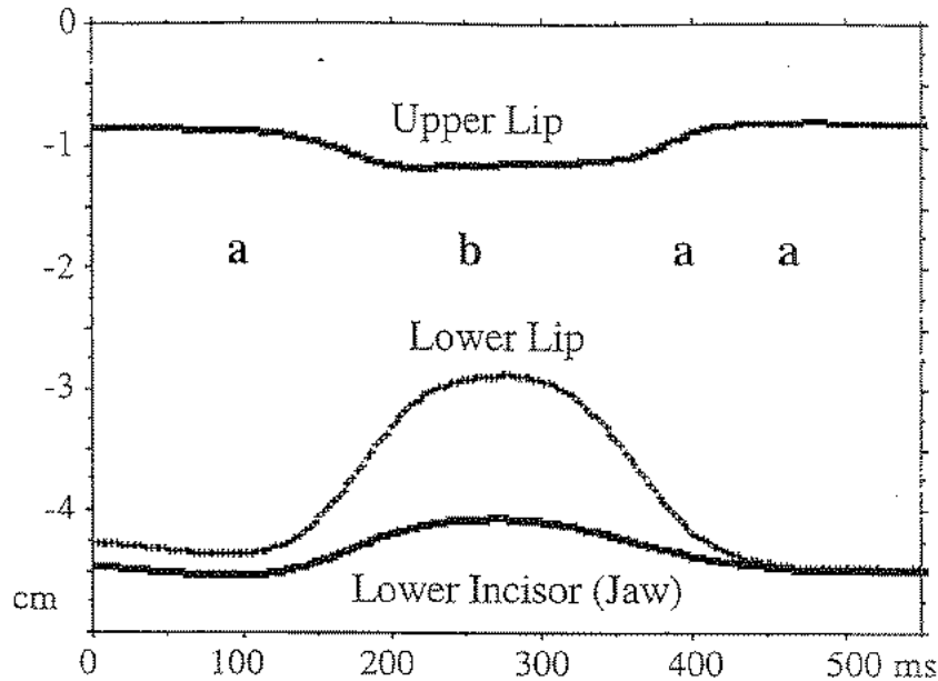
Figure 2.4 Mean vertical movement trajectories over time of the upper and lower lips and the jaw during ten repetitions of the Ewe word abaa 'mat' (from Maddieson 1993). Electromagnetic receivers were placed on the outside surface of the lips, hence a gap remains between them even during closure.
