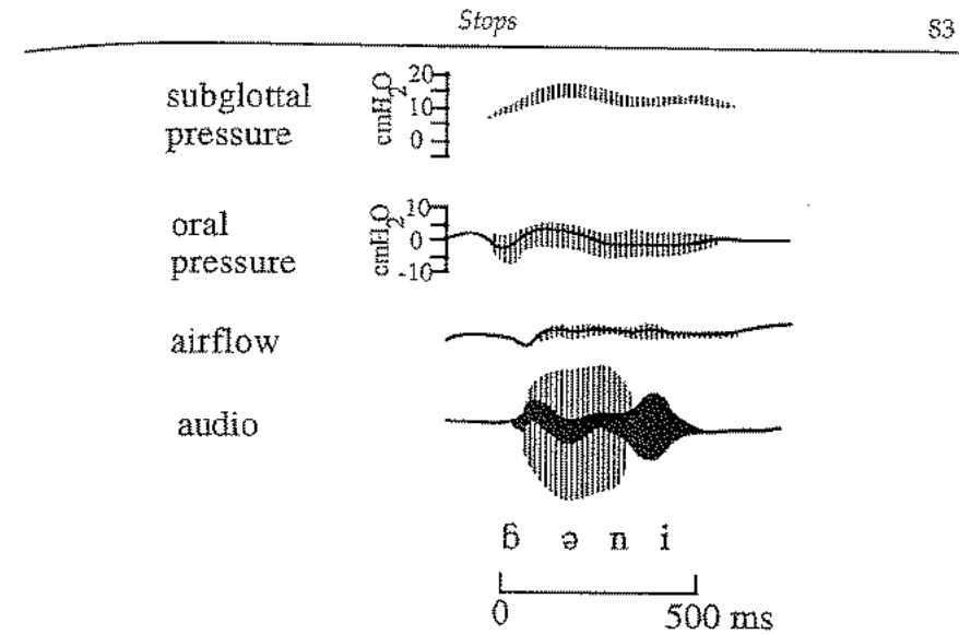
Figure 3.17 Aerodynamic data (based on Nihalani 1974) for the Sindhi implosive ɓ in the word ɓəni.
