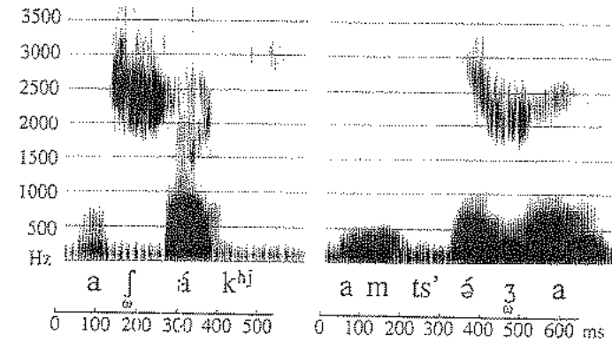
Figure 10.1 Abkhaz "bilabial-palatal" fricatives in the words \text{afak}^{\text{h}} and \text{amts}'\text{əza} spoken by a male speaker of the Bzyb dialect.
