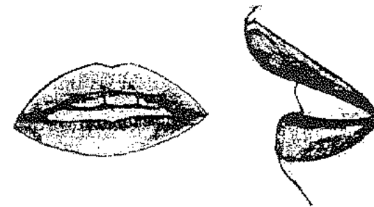
Figure 5.4 The tip of the tongue protruded between the teeth in \theta as in thief as pronounced by a speaker of Californian English.
