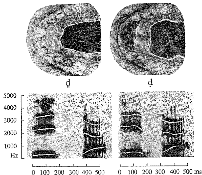
Figure 2.10 Spectrograms and palatograms illustrating the difference between laminal denti-alveolar \text{ḍ} and apical retroflex \text{d̠} in Ewe in the phrases \text{é ḍà} 'he throws' and \text{é d̠à} 'he cooks', based on Ladefoged (1968).
