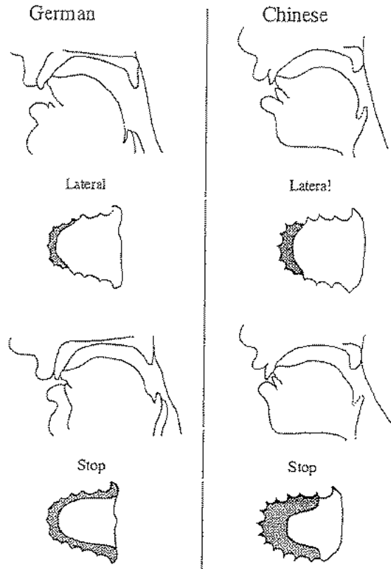
Figure 6.1 X-ray tracings and palatograms comparing articulatory positions for l and t in German and Standard Chinese (based on data in Wängler 1961, and Zhou and Wu 1963 respectively).
