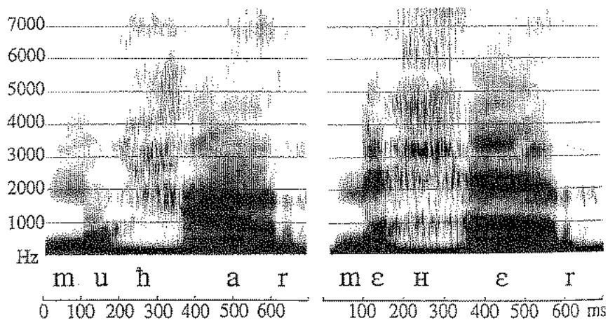
Figure 5.23 Spectrograms of the Agul words muhar 'barns', and mɛɸer 'wheys' spoken by a male speaker of the Burkikhan dialect.
