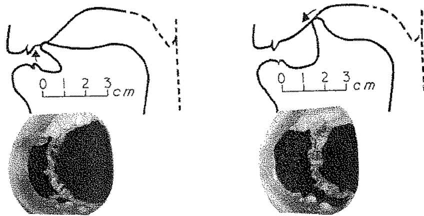
Figure 7.20 Palatograms (retouched) and deduced tongue positions in Hausa r and ɽ in the words bàrà: and báɽà: spoken by a male speaker from Zaria (from Ladefoged 1968).
