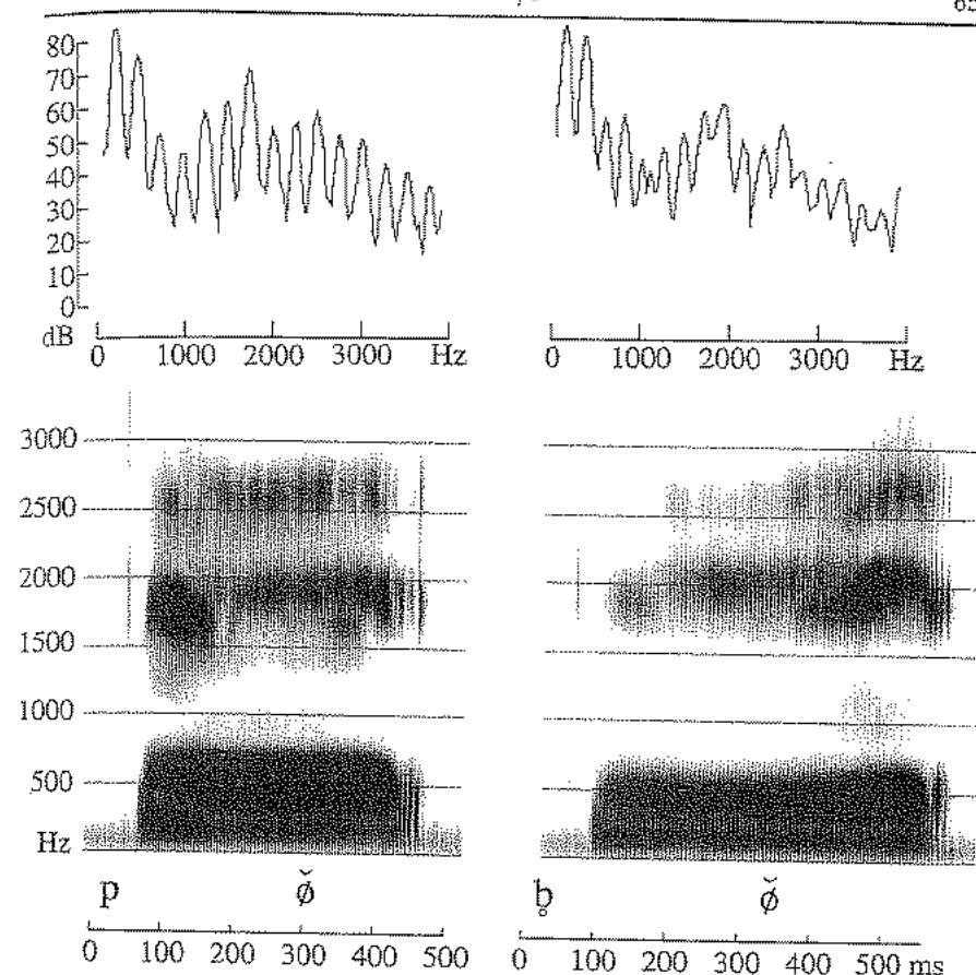
Figure 3.9 Spectrograms and power spectra illustrating the difference between Wu Chinese unaspirated stops. The words are pə 'half' and ḅə 'bowl' spoken by a female speaker from Shanghai.
