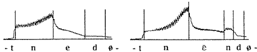
Figure 4.1 Difference in nasal airflow in French nez 'nose' and nain 'dwarf' spoken in the frame Dites deux fois , adapted from Cohn (1990: 110).
