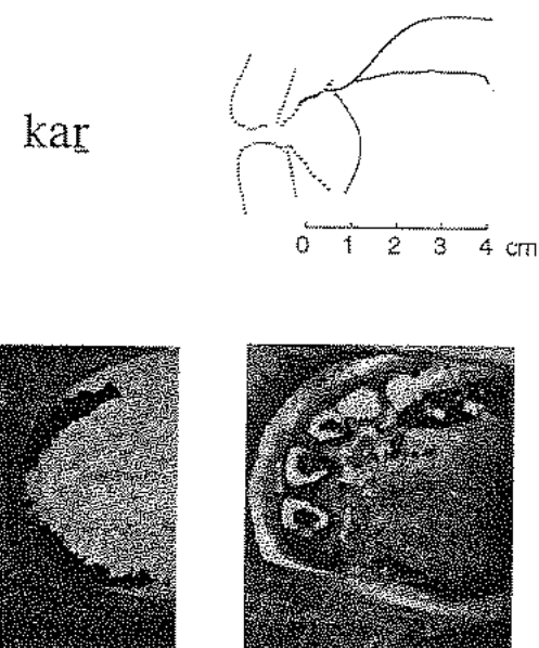
Figure 7.7 Palatogram, linguogram and reconstructed tongue position of the trill in the Toda word kar 'juice'.
