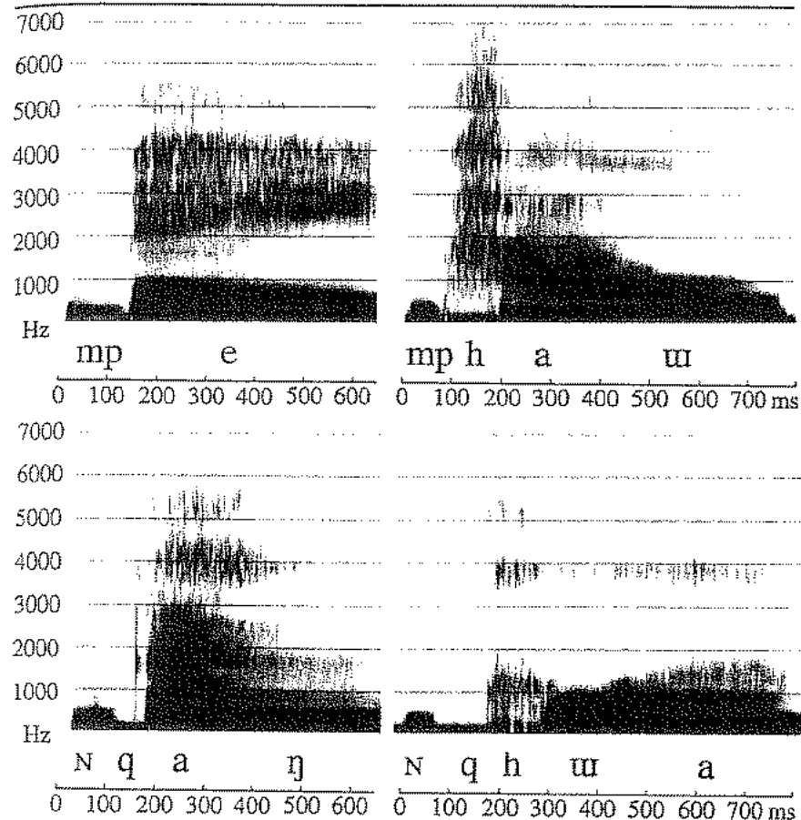
Figure 4.14 Spectrograms illustrating voiceless unaspirated and voiceless aspirated bilabial and uvular prenasalized stops as pronounced by a female speaker of Hmong Daw. The words are mpe 'name', nphau 'turbulent', nqan 'thatch' and nqhua 'dried up'.
