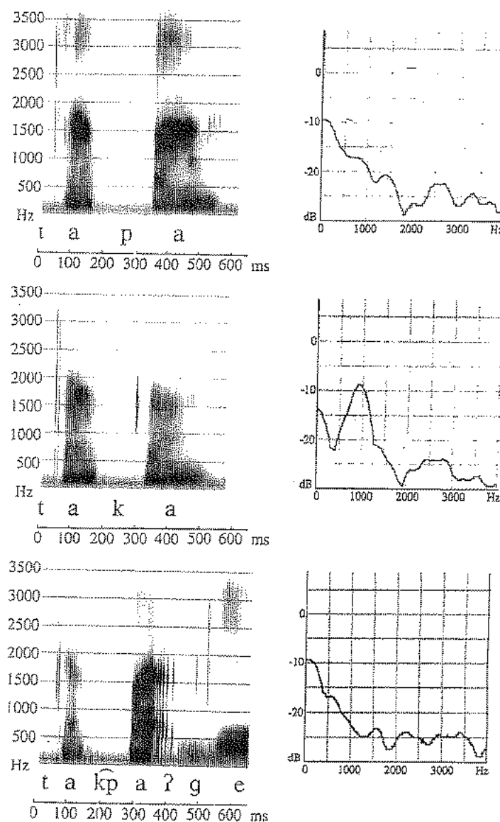
Figure 10.5 Spectrograms and stop burst spectra of Dedua words contrasting p , k and \widehat{k}p .
