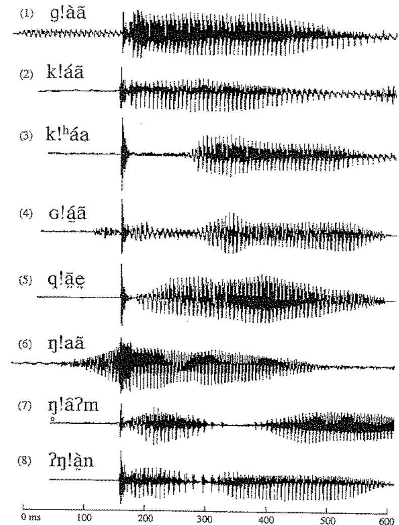
Figure 8.10 Waveforms showing the first eight alveolar clicks in IXóó in table 8.4.
