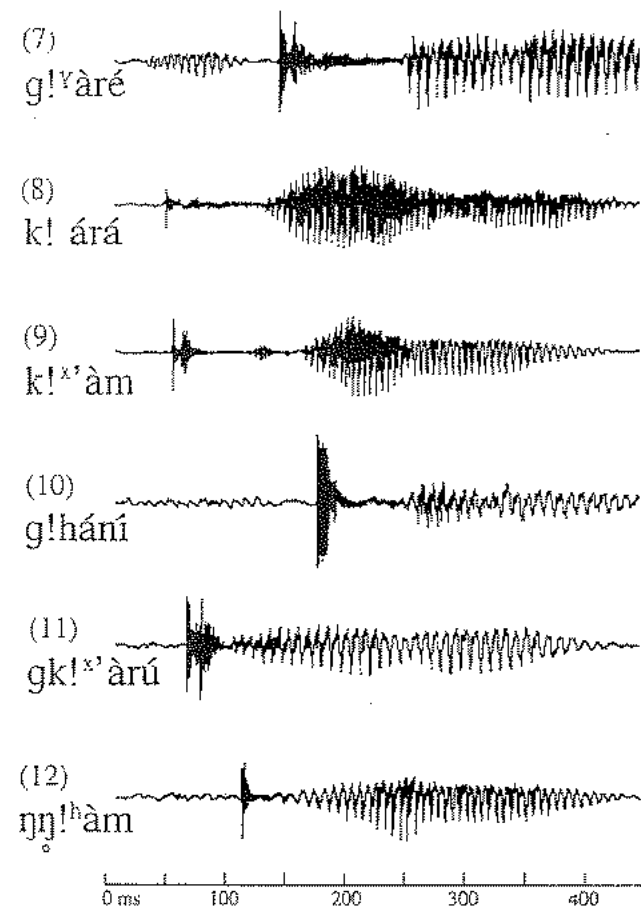
Figure 8.20 Waveforms of the last six Zhuǀ'hōasi alveolar clicks in table 8.5.
