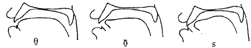
Figure 5.5 Tracings from x-rays of Icelandic non-sibilant alveolar fricatives \theta as in \theta aki \eth 'roof', and \eth as in va \eth an 'whence', compared with the sibilant alveolar s as in sunnar 'proved' (based on Pétursson 1971).
