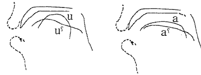
Figure 9.24 X-ray tracings of plain and pharyngealized vowels in IX66 (based on data in Traill 1985).
