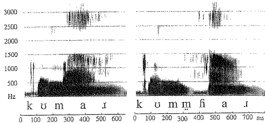
Figure 4.3 Spectrograms illustrating modally and breathy voiced nasals in Hindi in the words kumar 'boy' and konar 'potter' respectively. The transcription below the spectrogram shows additional phonetic detail.
