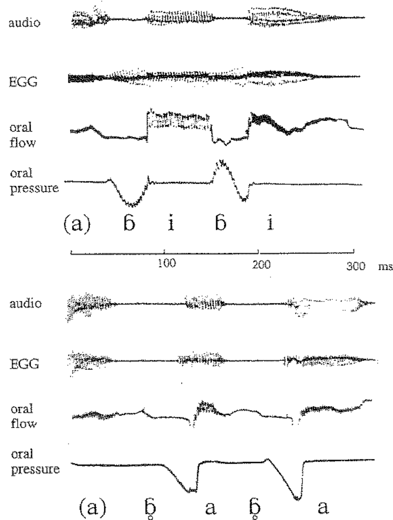
Figure 3.21. Aerodynamic records of Lendu implosives. In the words (a) biḽi 'eaten by insects', and (a) ḽáḽá 'attached to'. From data supplied by Demolin (personal communication).
