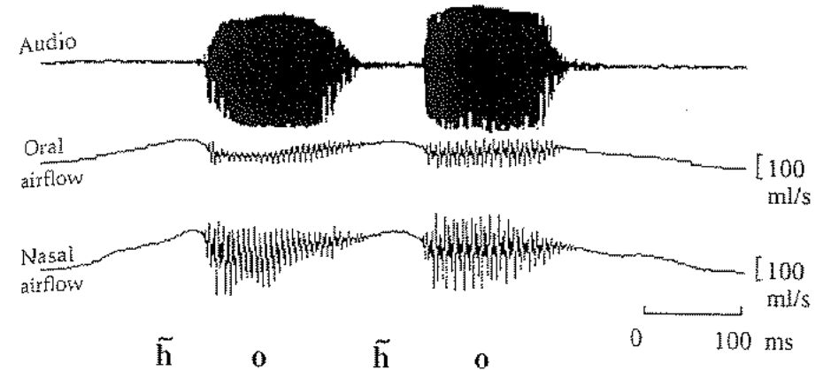
Figure 4.18 Aerodynamic records of voiceless glottal fricatives in the Kwangali word h̃õho shenho 'devil's thorn'.
