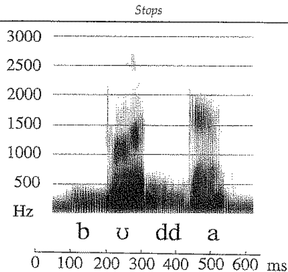
Figure 3.1 Spectrogram of the Ilwana word budda 'pelican' showing vocal fold vibration during both utterance-initial b and intervocalic geminate dd .
