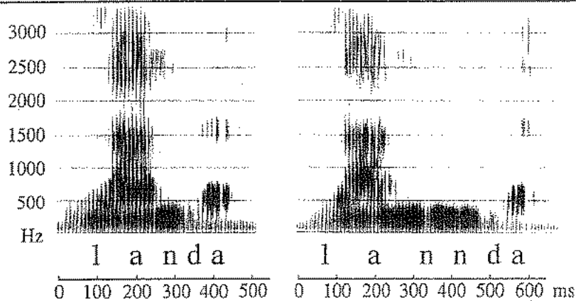
Figure 4.10 Spectrograms of Sinhala words contrasting 'prenasalized stop' in lan n da 'blind' and heterosyllabic nasal + stop sequence in lan.nda 'thicket'.
