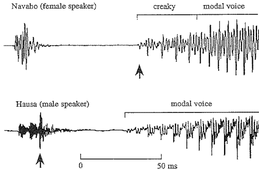
Figure 3.15 Waveforms illustrating differences between Navaho and Hausa velar ejective stops. The arrows indicate the releases of the glottal closures.
