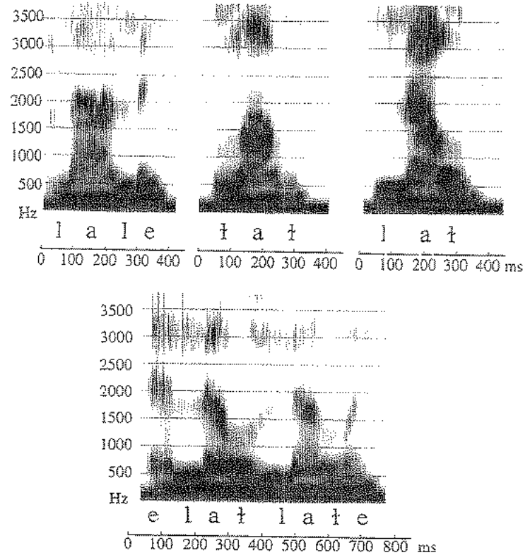
Figure 10.22 Marshallese late 'check' vs tat 'knock' vs lat 'earth' vs elate 'he's a down-to-earth person'.
