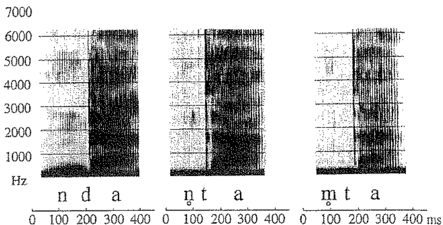
Figure 4.15 Spectrograms illustrating voicing assimilation in homorganic and heterorganic nasal + stop sequences in Bura in the words /nda/ 'cock', /nta/ 'tear (vb.)', /mta/ 'death'.
