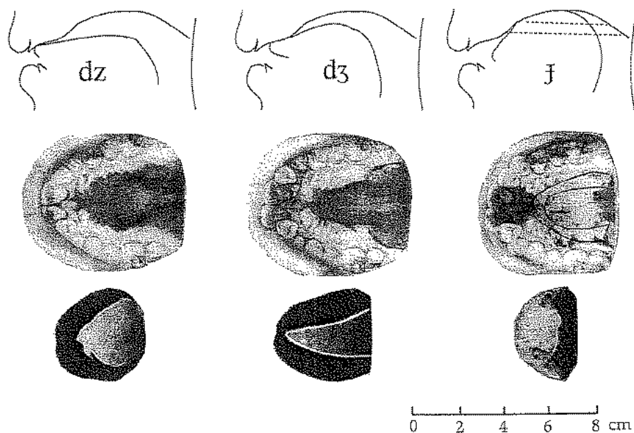
Figure 2.14 Palatograms, linguagrams, and inferred articulatory positions of laminal denti-alveolar, laminal palato-alveolar, and palatal stops in the Ngwo words édzé 'dance', dʒé (a species of fruit), éjé 'postpone' (based on Ladefoged, 1968). The contact area on the roof of the mouth is the area from which the marking medium has been wiped away. The dotted lines on the palatal sagittal section correspond to the (solid) contour lines superimposed on the palatogram.
