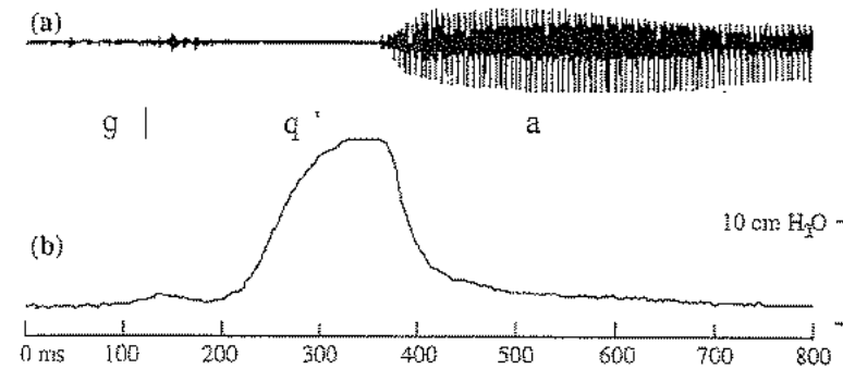
Figure 8.16 (a) Audio waveform and (b) pharyngeal pressure in a voiced dental click followed by a uvular ejective.
