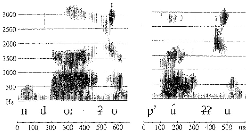
Figure 2.18. Spectrograms of intervocalic single and geminate ʔ in the Dahalo words nd6:ʔo 'floor' and p'6ʔʔu 'pierce'.
