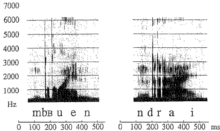
Figure 4.17 Spectrograms illustrating contrasting prenasalized alveolar and bilabial stops with trilled release in Kele in the words ndrai 'your blood' and mbu en 'its fruit'.
