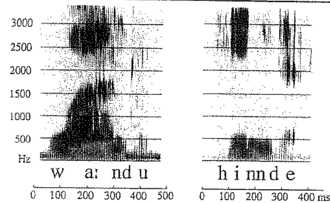
Figure 4.12 Spectrograms illustrating 'prenasalized stop' and geminate nasal + stop in Fula in the words wa:ndu 'monkey' and hinnde 'steamer'.
